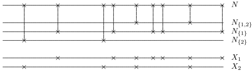
Figure 1: Representation of counting processes of Lévy type
