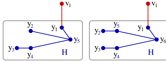
FIGURE 3. Small graphs, \delta = 1, \Delta = 3 in Lemma 12
