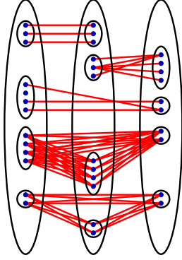
FIGURE 1. A graph from class \mathcal{P}'_3 .
