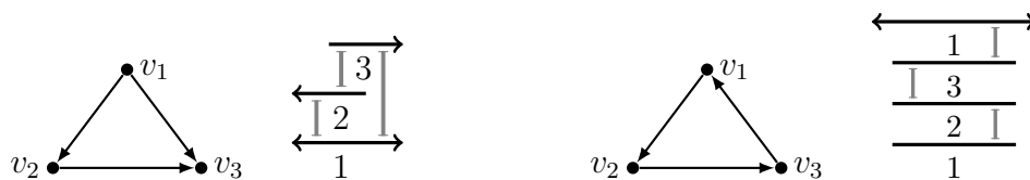
Figure 4.1: Layouts of 3-tournaments.
