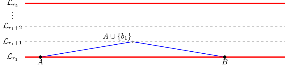
Figure 1: the shortest A - B path when k = 1
