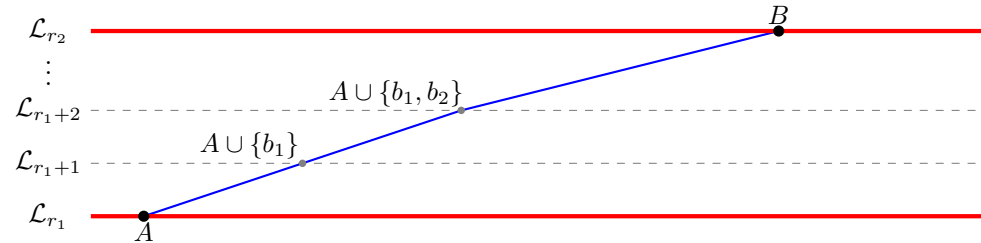
Figure 3: the shortest A - B path when A \setminus B = \emptyset
