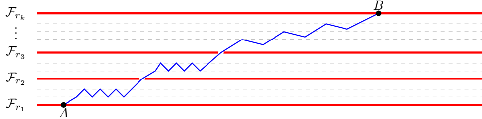
Figure 5: the constructed A - B path
