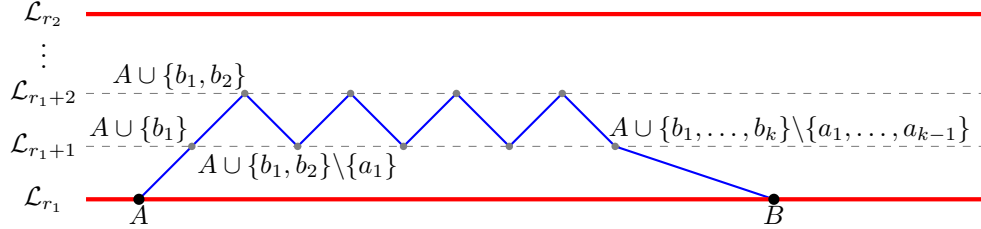
Figure 2: the shortest A - B path when k \geq 2
