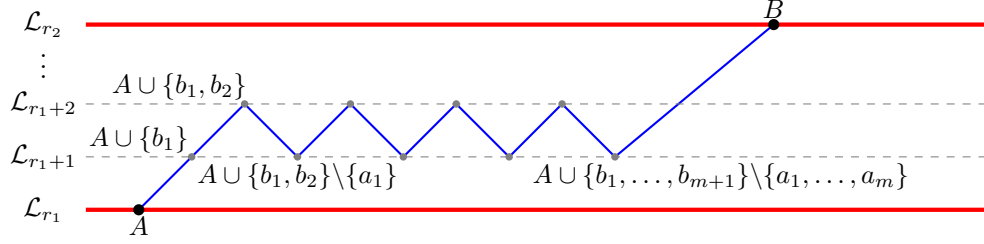
Figure 4: the shortest A - B path when A \setminus B \neq \emptyset
