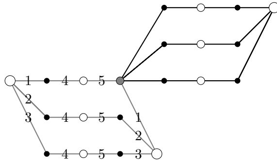
Figure 1: A graph H(3) with larger vertices being poles in the respective copies of theta graphs as well as a nice coloring of one theta graph
