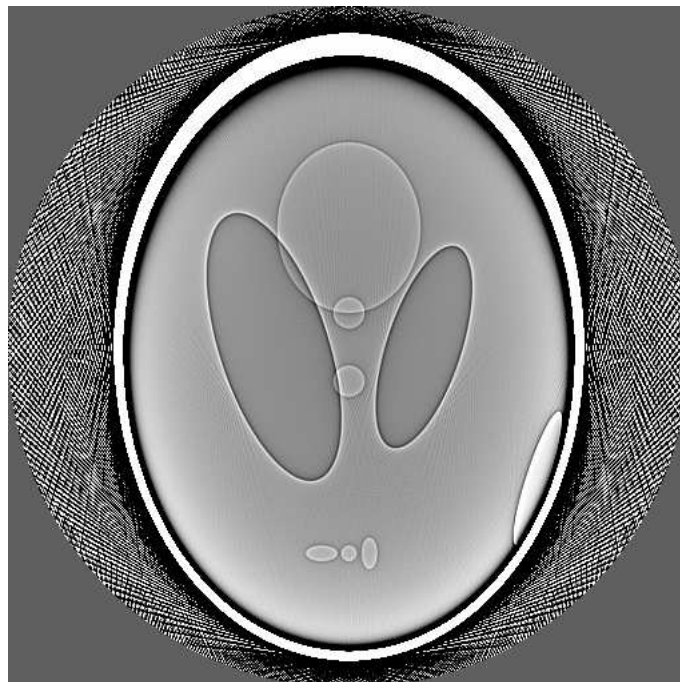
\Lambda f (numerische Approximation)
