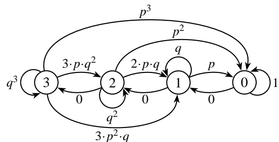
Abb. 5: Prozessdiagramm; p = \frac{1}{6} , q = \frac{5}{6}
