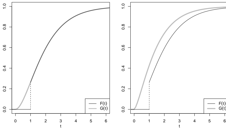
Fig. 1 Cdf's F and G as defined in Example 1, in the left panel both with shape parameter 2, in the right panel F with shape parameter 2 and G with 1.5. In both panels F \leq_c G holds, in the right one even in a strict sense.
