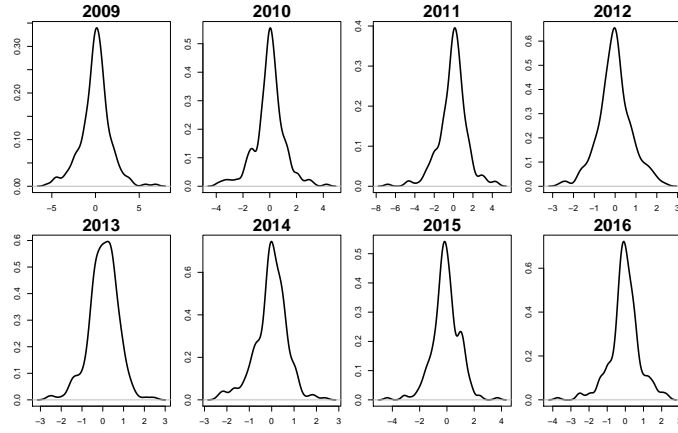
Figure 10: Estimated densities for the data sets of residuals divided by year.
