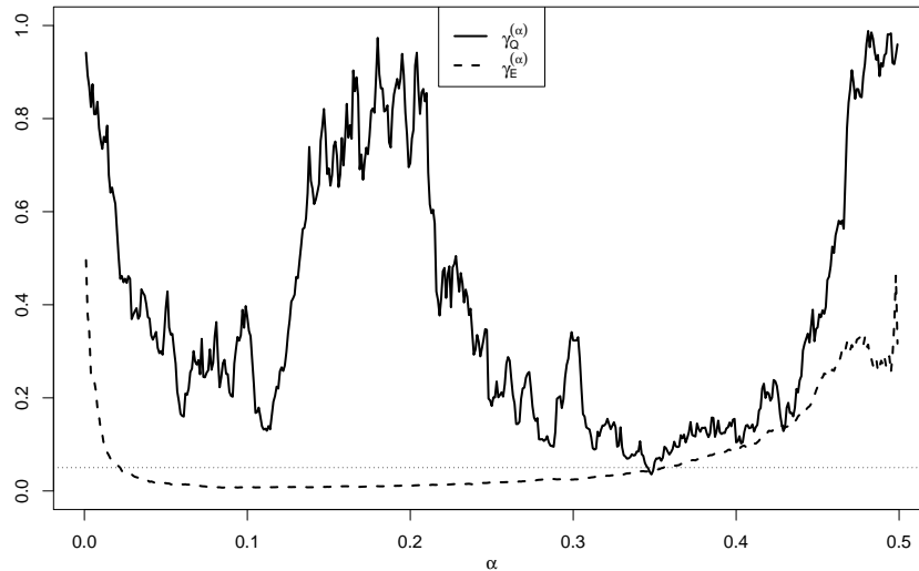
Figure 9: p -values of tests on nullity of the quantile and expectile skewness as a function of the parameter \alpha .
